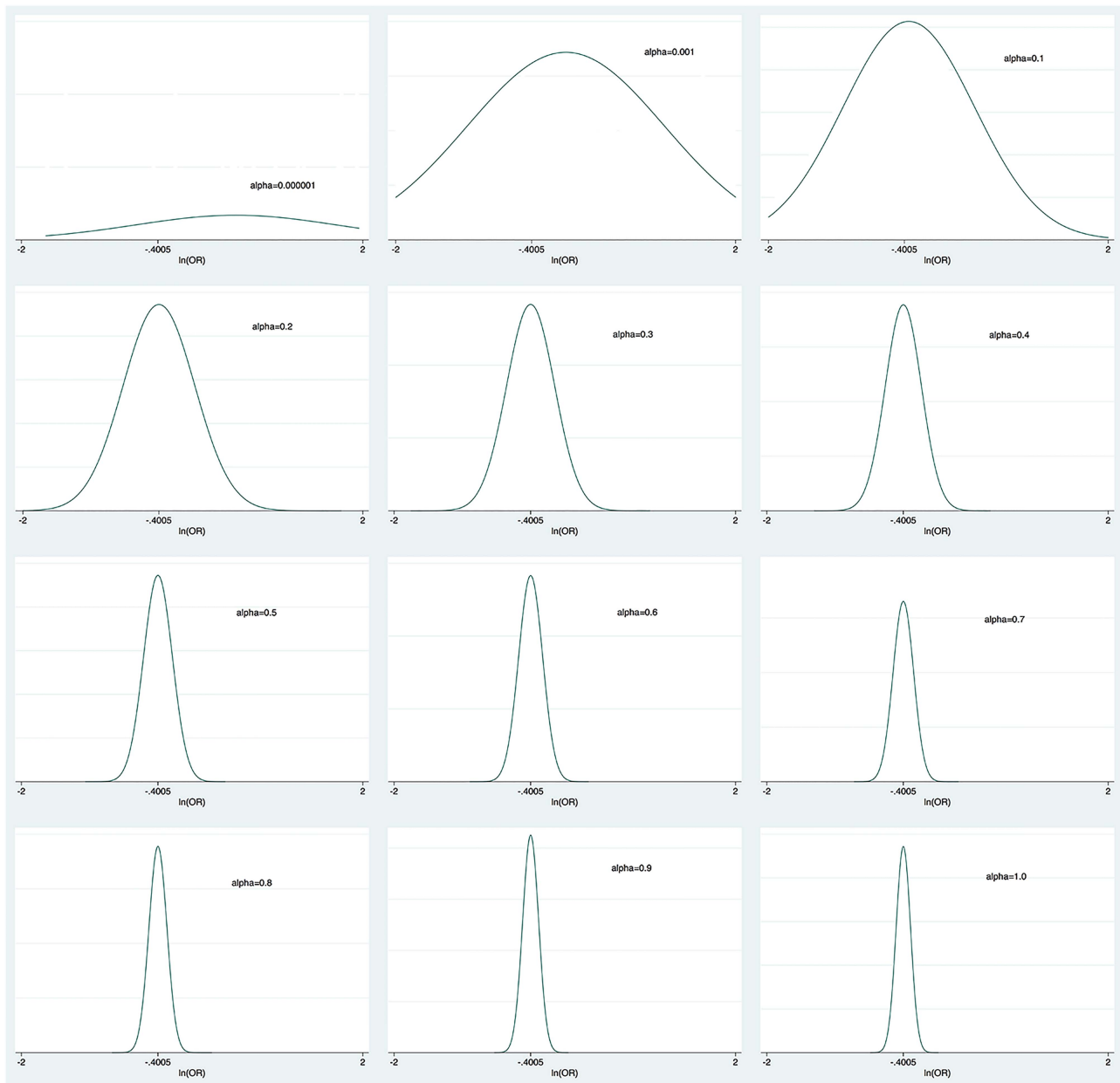
Figure 6 Prior distribution derived by discounting observational evidence with \alpha from 0.000001 to 1. The plots show that the precision of prior increases with increasing \alpha values.
