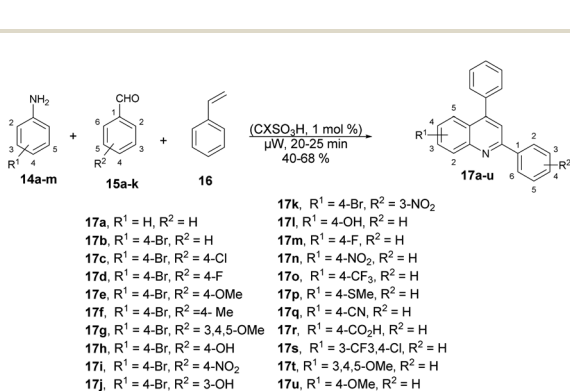
Scheme 6 Synthesis of various derivatives of quinolines 17a-u .
