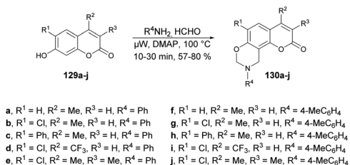
Scheme 47 Synthesis of coumarin[8,7-e][1,3]oxazine derivatives 130a-j.
