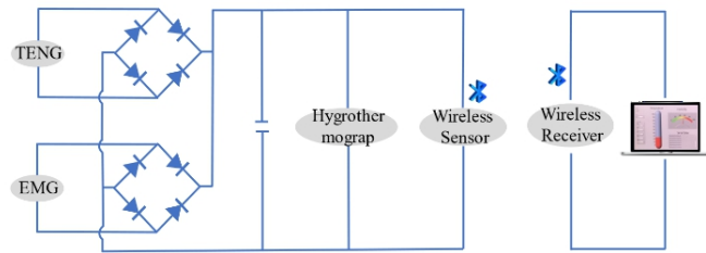
Self-powered wireless temperature and humidity sensing node
