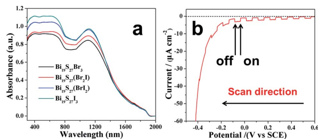
Fig. 6 (a) UV-vis-NIR diffuse-reflectance spectra (DRS) of the \text{Bi}_{19}\text{S}_{27}(\text{Br}_{3-x}\text{I}_x) ( 0 \leq x \leq 3 ) NWs, (b) transient photocurrent response of the \text{Bi}_{19}\text{S}_{27}(\text{BrI}_2) NWs.
