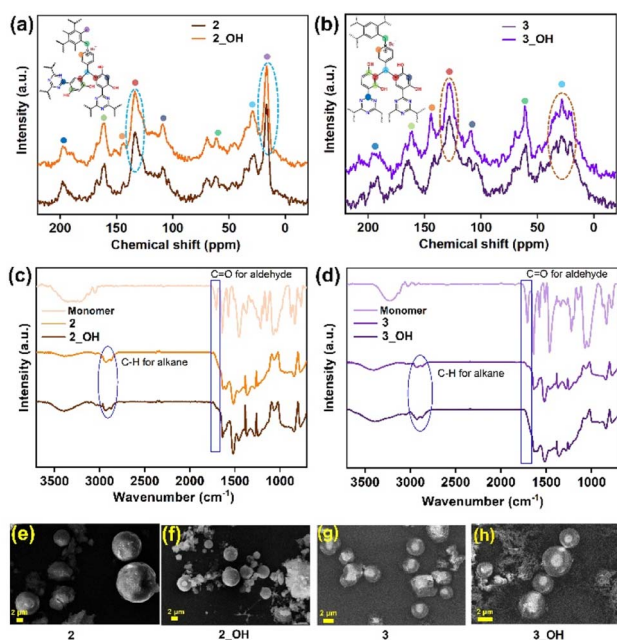
Fig. 1 (a) 13 C-CPMAS spectra of 2 and 2_OH ; (b) 3 and 3_OH ; (c) FTIR spectra of Aldehyde monomers, 2 , and 2_OH ; (d) 3 , and 3_OH ; (e) and (f) FESEM images of 2 and 2_OH ; (g) and (h) FESEM images of 3 and 3_OH .
