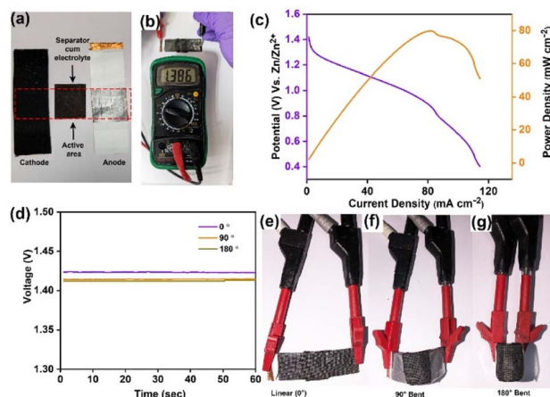
Fig. 5 (a) Components of F-RZABs showing cathode, anode and electrolyte; (b) digital photograph of F-RZAB and multimeter device respectively; (c) recording of the current ( I )–voltage ( V ) polarization plot for F-RZAB; (d) comparative OCV acquired at different bending angles, illustrating the device flexibility; (e–g) digital photograph of the flexible device at various angles ( 0^\circ , 90^\circ , and 180^\circ ).
