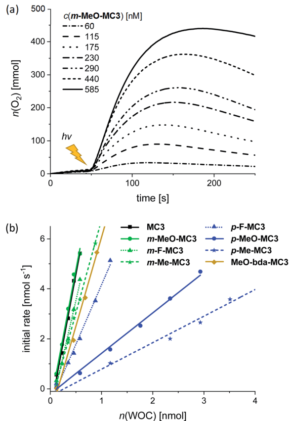
Fig. 5 (a) Concentration-dependent oxygen evolution curves of m -MeO-MC3 in MeCN/ \text{H}_2\text{O} 1 : 1 (pH 7, phosphate buffer), c(\text{PS}) = 1.5 \text{ mM} , c(\text{Na}_2\text{S}_2\text{O}_8) = 37 \text{ mM} . The lighting symbol indicates the start of sample irradiation at t = 50 \text{ s} . (b) Initial rates of all macrocycles with linear regression for the determination of averaged TOF.
