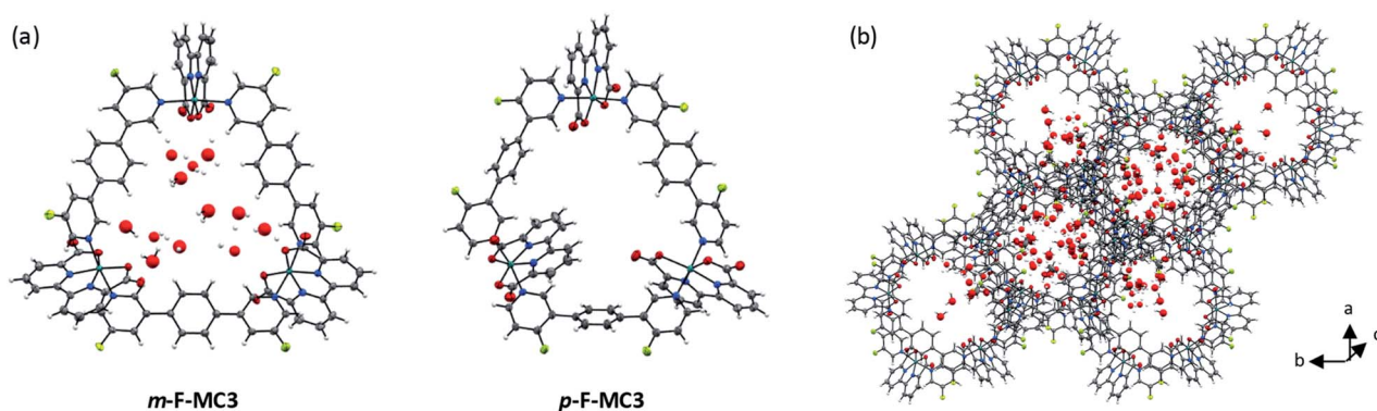
Fig. 2 (a) Crystal structures of m - F-MC3 and p - F-MC3 determined by single crystal X-ray diffraction (ORTEP diagram with thermal ellipsoids set at 50% probability; grey: carbon, white: hydrogen, red: oxygen, blue: nitrogen, turquoise: ruthenium, green-yellow: fluorine). The crystals were grown from a DCM/methanol solvent (not dried) mixture. (b) Crystal packing of m - F-MC3 , view along axis c with water and methanol molecules in the pores. a = 23.4927(5) Å, b = 23.4927(5) Å, c = 32.5166(7) Å, \alpha = 90^\circ , \beta = 90^\circ , \gamma = 120^\circ .
