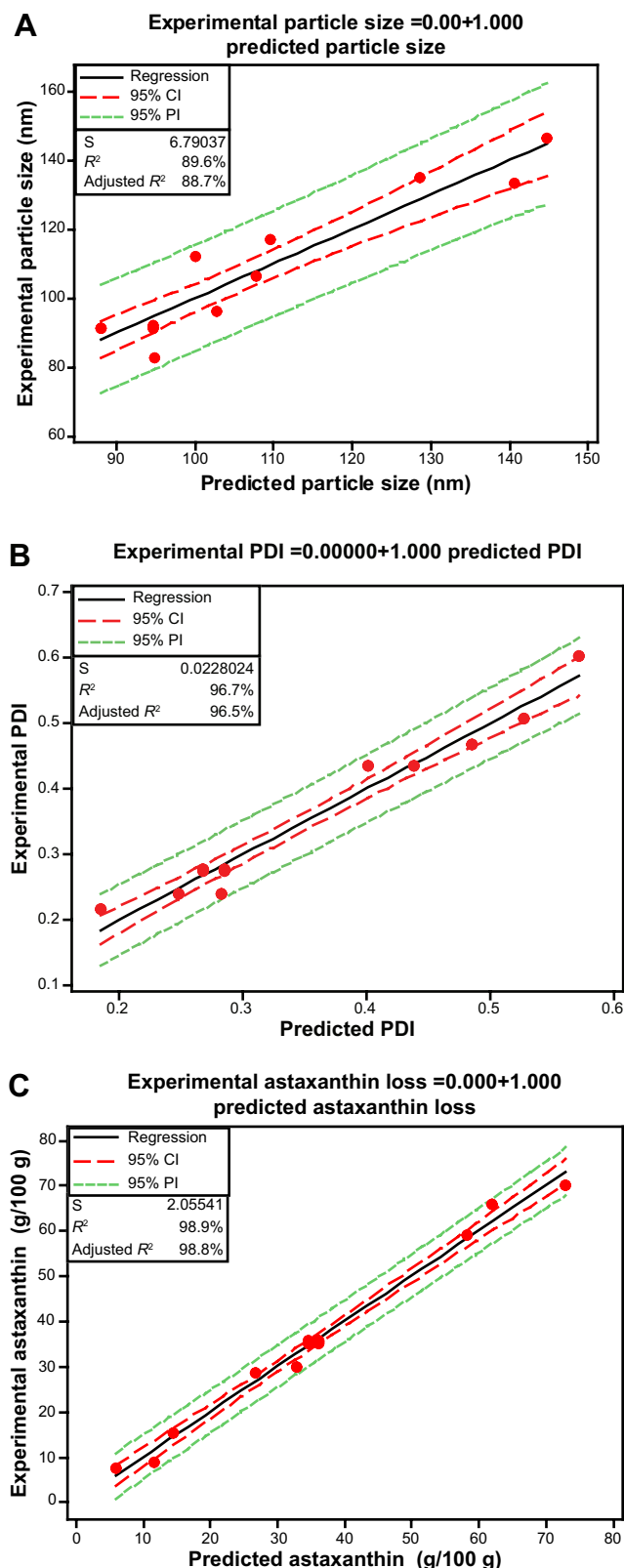
Figure 3 Fitted line plots between the experimental and predicted values for (A) mean particle size, (B) PDI and (C) astaxanthin loss; dashed lines (- -) and dotted lines (⋯) show 95% CI and 95% PI, respectively.
