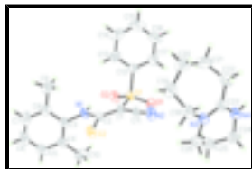
Fig. 1. View of the title compound with atomic numbering scheme. All atoms are shown with displacement ellipsoids drawn at the 50% probability level.
