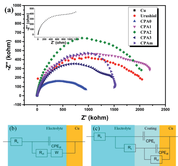
Fig. 8 Nyquist plots for copper, urushiol and urushiol analogues coating in 3.5 wt% NaCl solution at 25 °C (a) and equivalent circuit model used for fitting EIS dates of bare Cu (b) and coated Cu (c).
