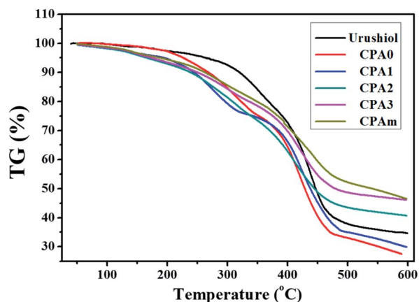
Fig. 5 TG analysis of the coatings of urushiol and urushiol analogues.
