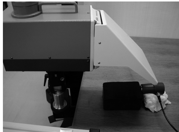
Fig. 1. Setting for thermometry
