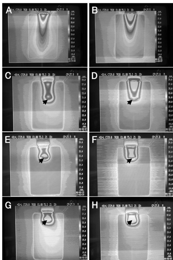
Fig. 2. The temperature distribution of the phantom irradiated with 1 MHz (A, C, E, G) and 3 MHz (B, D, F, H) continuous ultrasound for 5 minutes at 2.0 \text{ W/cm}^2 at distances between the bone and transducer of 5 cm (C, D), 3 cm (E, F), and 2 cm (G, H). The arrow shows the position of the bone (C–H)
