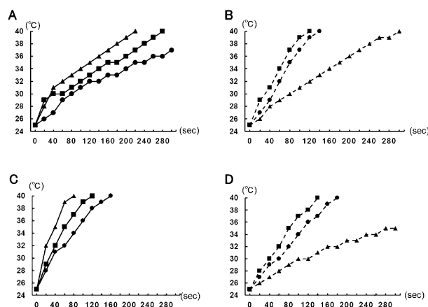
Fig. 3. The temperature around the bone and transducer. Graphs A and B show the temperature of the phantom irradiated by 1 MHz continuous ultrasound, and graphs C and D show the temperature for 3 MHz continuous ultrasound. The solid lines represent the temperature around the transducer (A, C). The dashed lines represent the temperature around the bone (B, D). The squares, circles, and triangles represent temperature at distances between the bone and transducer of 2 cm, 3 cm, and 5 cm.
