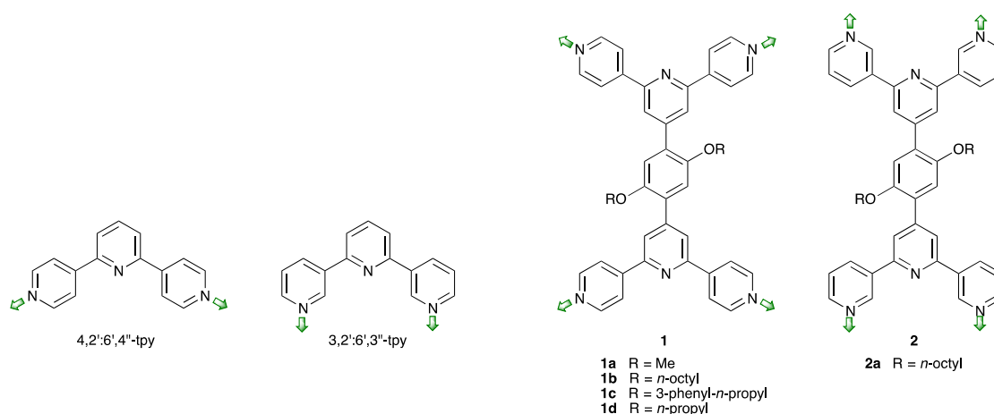
Scheme 2. Structures of 4,2':6',4''- and 3,2':6',3''-tpy of general ligand types 1 (with 4,2':6',4''-tpy units) and 2 (with 3,2':6',3''-tpy units), and structures of ligands 1a–1d and 2a . The green arrows show the vectorial orientation of the lone pairs involved in formation of the coordination network.
