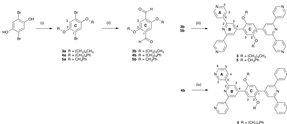
Scheme 4. Synthetic routes to 3–5 with numbering for NMR spectroscopic assignments in the experimental section; CH 2 units in alkyloxy chains are labelled a, b, c . . . etc. starting at the OCH 2 unit and the terminal phenyl rings are labelled D. Conditions: (i) RBr or benzyl chloride (see Materials and Methods), anhydrous K 2 CO 3 , dry DMF, 100 °C, 15 h; (ii) n BuLi, Et 2 O, 0 °C; DMF, warmed to room temperature, 15 h; (iii) 4-acetylpyridine, KOH, EtOH, aqueous NH 3 , room temperature, 15 h; (iv) 3-acetylpyridine, KOH, EtOH, aqueous NH 3 , room temperature, 15 h.
