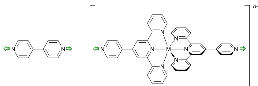
Scheme 1. An [M(\text{tpy})_2]^{n+} complex is considered as an expanded 4,4'-bpy.
