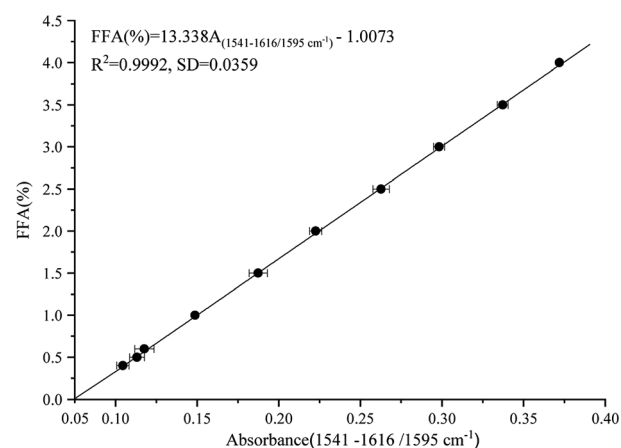
Fig. 2 Calibration of FFA contents versus peak areas of FFA measured at 1616\text{--}1541\text{ cm}^{-1} and referenced to 1595\text{ cm}^{-1} as baseline, which was obtained from the spectra of soybean oil spiked with varying amounts of FFA.
