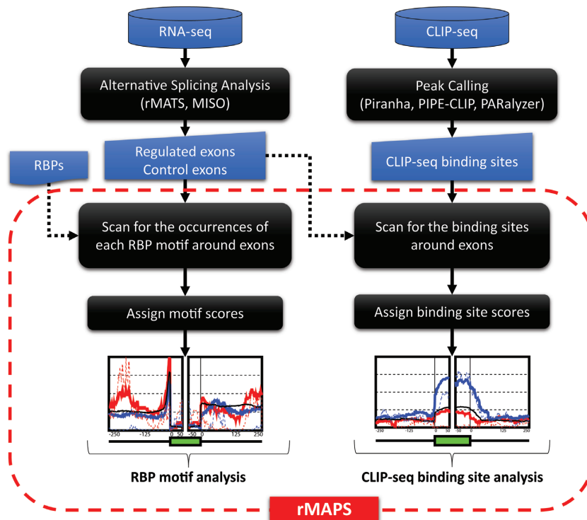
Figure 2. Overall workflow of rMAPS. The RBP motif analysis takes the AS analysis results from RNA-seq data, then scans for the occurrences of the known RBP motifs around the differentially regulated alternative exons to generate an RNA map for each RBP. Similarly the CLIP-seq binding site analysis generates an RNA map using the signals of CLIP-seq binding sites around the differentially regulated alternative exons.
