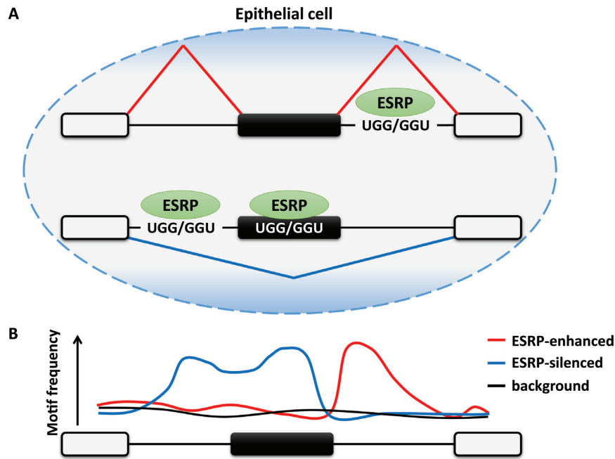
Figure 1. Binding-site-position dependent regulation of epithelial specific AS by ESRP proteins. The solid black exon in the middle is the ESRP regulated exon. (A) ESRP generally enhances splicing when it binds to the downstream intron while it suppresses splicing when it binds to the upstream intron or within the regulated exon. (B) A schematic RNA map for the spatial distribution of the ESRP consensus motif around different categories of alternative exons. The red line represents the enriched ESRP motif in the downstream intron of ESRP-enhanced exons, while the blue line represents the enriched ESRP motif in the upstream intron and within the exon of ESRP-silenced exons. The black line represents the motif density for background (non-regulated) exons.
