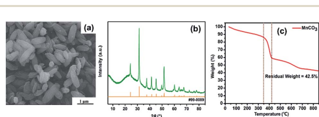
Fig. 2 SEM image (a), XRD pattern (b) and the TGA curve of the MnCO 3 particles (c).
