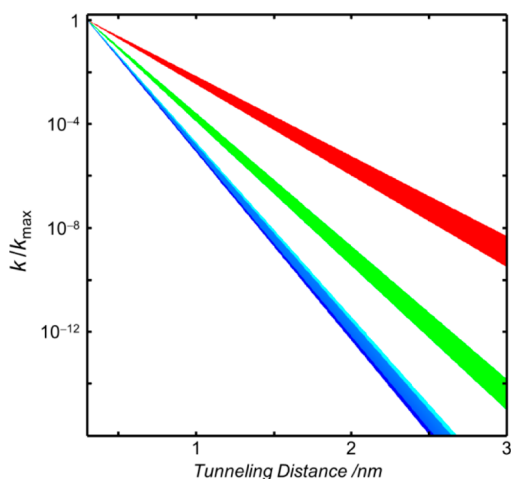
Figure 3. Distance dependence of rate constants for electron tunneling through solvent glasses (2-MTHF, blue; 25% aqueous \text{H}_2\text{SO}_4 , cyan; toluene, green) and across oligoxyethylene bridges (red). 38,39
