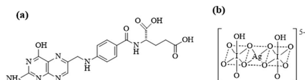
Fig. 1 Chemical structure of (a) folic acid and (b) Ag(III) complex.
