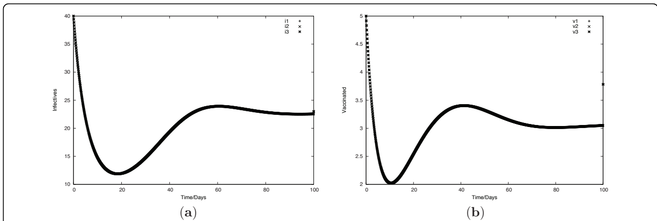
Figure 4 Optimalty effect when the weight constraint for the infected population varies and media has an adverse effect on the vaccine. Graphical representation of the optimality system when media coverage has an adverse effect on the vaccination rate and when the weight constraint for the infected population varies. (a) Graph of infectives. (b) Graph of vaccinated individuals. Initial conditions: S(0) = 20.0 , I(0) = 25.0 , V(0) = 50.0 , R(0) = 40.0 . The value of the weights used are (i) B1 = 0.0025 corresponds to variables with subscript 1 (++), (ii) B1 = 25.0 corresponds to variables with subscript 2 (xx), (iii) B1 = 250000.0 corresponds to variables with subscript 3 (**). The value B2 = 0.0025 is kept constant in all three cases.
