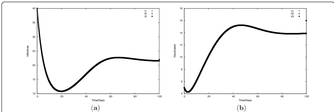
Figure 2 Optimality effect when the weight constraint for the infected population varies and media has a beneficial effect on the vaccine. Graphs of the optimality system when media coverage has a beneficial effect on the vaccination rate and when the weight constraint for the infected population varies. (a) Infected individuals. (b) Vaccinated individuals. Initial conditions: S(0) = 20.0 , I(0) = 25.0 , V(0) = 50.0 , R(0) = 40.0 . The value of the weights used are (i) B_1 = 0.0025 corresponds to variables with subscript 1 (++), (ii) B_1 = 25.0 corresponds to variables with subscript 2 (xx), (iii) B_1 = 250000.0 corresponds to variables with subscript 3 (**). The value B_2 = 0.0025 is kept constant in all three cases.
