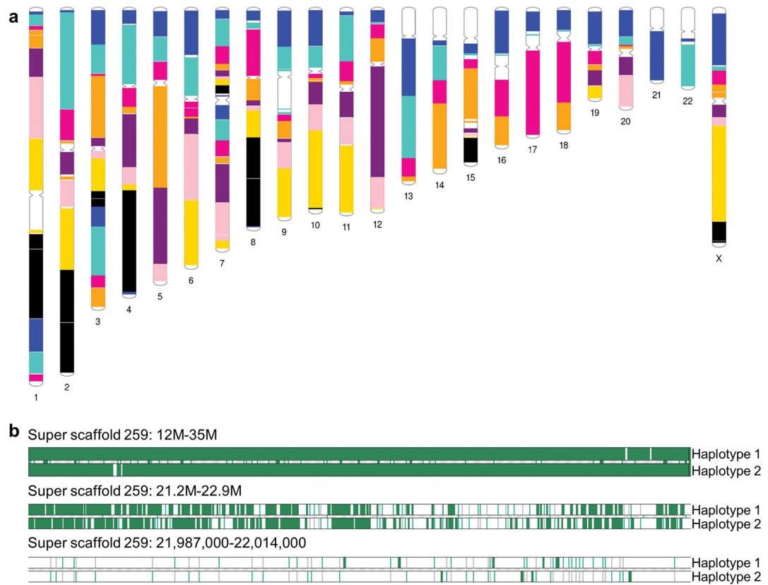
Figure 3. Alignment and phasing of the hybrid assembly
