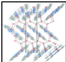
Fig. 3. The three-dimensional packing of the title compound viewed along the a axis, showing the hydrogen bonds with dashed lines.
