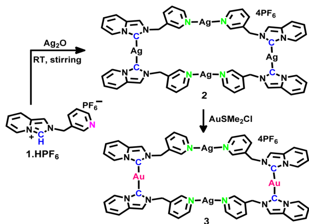
Scheme 1 Site selective metallation of 1 HPF 6 with Ag(I) and Au(I). The letters surrounding 1 refer to the NMR assignments; see the Experimental section.
