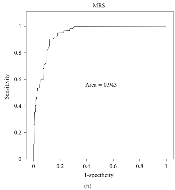
FIGURE 3: Receiver operator characteristic (ROC) curve of DWI (a) and MRS (b) for differentiating tumor tissue from normal tissue. The analysis included all 300 tissue probes irrespective of the ROI.
