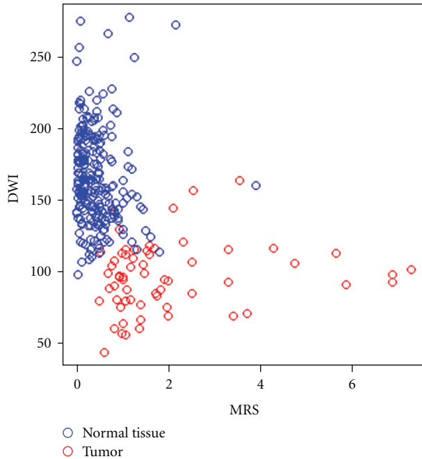
FIGURE 4: Scatter plot of DWI versus MRS in normal tissue probes and tumor-positive tissue probes.
