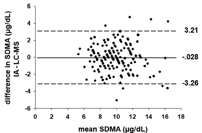
FIGURE 2 Bland-Altman scatter plot illustrating bias and 95% limits of agreement for serum symmetric dimethylarginine (SDMA) concentrations measured by liquid chromatography-mass spectroscopy (LC-MS) and immunoassay (IA) in 165 serum samples collected from healthy draft horses
