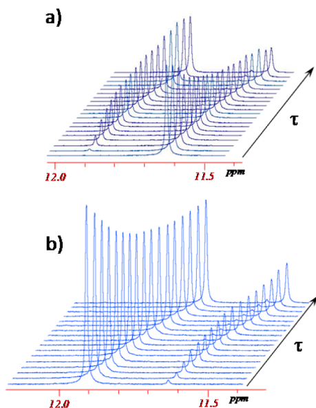
Figure 3. Evolution of ^1\text{H} NMR spectra (500 MHz) in the NH region of the [ trans-RuCl 4 (NO)(Hind)] - (a) and [ cis-RuCl 4 (NO)(Hind)] - (b) isomers as a function of time ( \tau = [0-3] \times 10^5 s) at 100 °C in \text{C}_2\text{D}_2\text{Cl}_4 ( C_{0(\text{trans})} = 14.5 mmol/L; C_{0(\text{cis})} = 13.7 mmol/L) showing the formation of the cis and trans isomers, respectively.
