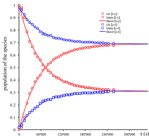
Figure 5. Time evolution of populations for [ cis-RuCl 4 (NO)(Hind)] - (O) and [ trans-RuCl 4 (NO)(Hind)] - (□) isomers at 100 °C in \text{C}_2\text{D}_2\text{Cl}_4 for cis to trans [ c-t ] (blue) and trans to cis [ t-c ] (red) isomerization processes. The solid lines are the best fits with activation parameters indicated in the text (for fitted plots at 90, 105, and 110 °C, see Supporting Information Figures S6 and S7).
