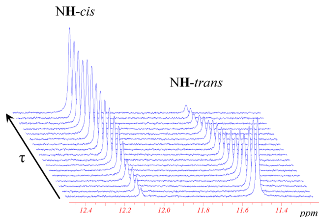
Figure 4. Evolution of ^1\text{H} NMR spectra (300 MHz) of the [ trans-OsCl 4 (NO)(Hind)] - isomer in the NH region as a function of time ( \tau = [0-3] \times 10^5 s) at 120 °C in \text{C}_2\text{D}_2\text{Cl}_4 ( C_0 = 15.26 mmol/L) showing the formation of the cis isomer (for complete aromatic region spectrum, see Supporting Information Figure S5).
