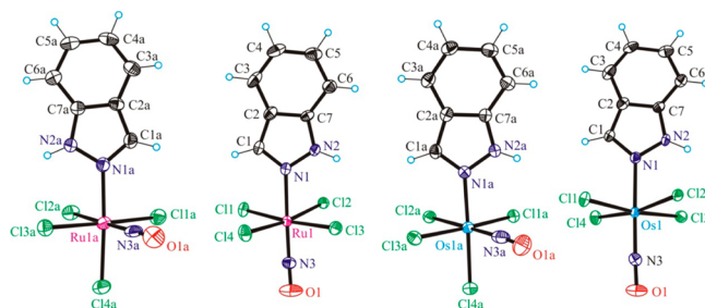
Figure 1. ORTEP views of the [\text{cis-RuCl}_4(\text{NO})(\text{Hind})]^- , [\text{trans-RuCl}_4((\text{NO})(\text{Hind}))]^- , [\text{cis-}[\text{OsCl}_4(\text{NO})(\text{Hind})]^-] , and [\text{trans-}[\text{OsCl}_4(\text{NO})(\text{Hind})]^-] complex anions in 1–4 (from left to right). Thermal ellipsoids are drawn at the 50% probability level.
