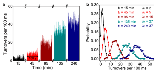
Figure 3. Single turnover stochastics of the oligomerization reaction monitored at the surface of the H-ZSM-5-P single crystal for 4 h in a 5.75 mM solution of FA. (a) Total number of detected turnovers per frame as a function of time. Each time interval is 100 s. Note the large time gaps between the measurements. (b) Poisson distributions of the corresponding color-coded trajectories presented in (a), including the Poisson parameter \lambda .
