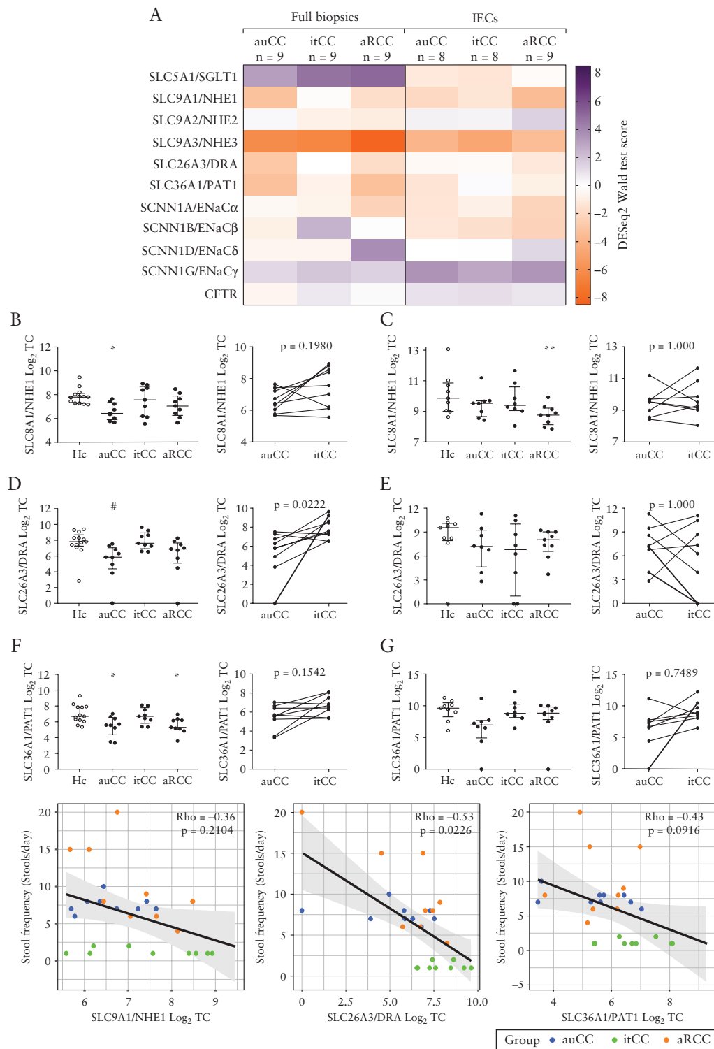
Figure 5. Ion channel expression is modestly decreased in CC colonic mucosa. [A] Heatmap showing normalized, \log_2 -transformed read counts [DESeq2 Wald statistic test scores] for the indicated channel genes in CC full biopsy samples and microdissected IECs. Samples were analysed by transcriptome-wide mRNA sequencing [RNA-seq]. SCNN1D did not reach the minimum threshold of 10 total reads in IEC samples [grey]. n = 8 –13 per group. [B–G] Transcript counts [TC] of NHE1 [B, C], DRA [D, E], and PAT1 [F, G] in all CC groups [left, median with interquartile range], and paired CC samples before [auCC] and during [itCC] successful treatment with budesonide [right]. Panels B, D and F correspond to full biopsy RNA-seq data, and panels C, E and G to IEC RNA-seq data. Sample number for full biopsy RNA-seq was n = 13 for Hc, and n = 9 for the CC full biopsy cohort; and for IEC RNA-seq was n = 9 for Hc and aRCC, and n = 8 for auCC and itCC. [H–J] Scatter plots showing the correlation of stool frequency per day with NHE1 [H], DRA [I] and PAT1 [J] \log_2 -transformed TC, as determined by RNA-seq, in all CC full biopsy samples. Spearman's rho and the adjusted p -value [FDR-corrected] are shown in the graph. The trend-line indicates the linear regression model with 95% confidence interval [grey]. Statistically significant differences relative to Hc samples are shown as * p < 0.05 and ** p < 0.01 ; statistically significant differences relative to itCC samples are shown as # p < 0.05 . au, active/untreated; aR, active/refractory; CC, collagenous colitis; Hc, healthy controls; it, inactive/treated; RNA-seq, RNA-sequencing; TC, transcript counts.
