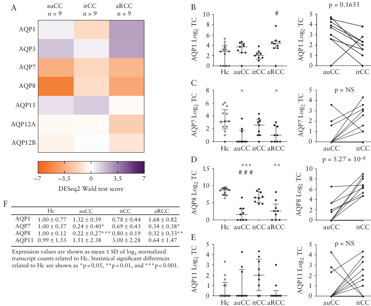
Figure 2. RNA-seq analysis confirming AQP8 modulation in CC colonic mucosa. [A] Heatmap showing normalized, log 2 -transformed read counts [DESeq2 Wald statistic test scores] for the indicated AQP genes in CC mucosal biopsy samples [ n = 13 Hc, and n = 9 per CC group]. Samples were analysed by transcriptome-wide mRNA sequencing [RNA-seq]. Datasets with < 10 total reads with a value of \geq 1 read were omitted. [B–E] Transcript counts [TC] of AQP1 [B], AQP7 [C], AQP8 [D] and AQP11 [E] in all CC groups [left, median with interquartile range], and paired CC samples [ n = 18 ] before [auCC] and during [itCC] successful treatment with budesonide [right]. p -values are FDR-adjusted; values above the significance threshold of 0.05 are shown as not significant [NS]. Sample number in all panels was n = 13 for Hc and n = 9 for CC cohorts. [F] Summarized AQP transcript counts, normalized to Hc. Expression values are shown as mean \pm SD of log 2 -transformed TC. Statistically significant differences relative to Hc samples are shown as * p < 0.05 , ** p < 0.01 and *** p < 0.001 ; statistically significant differences relative to itCC samples are shown as * p < 0.05 , and *** p < 0.001 . AQP, aquaporin; au, active untreated; aR, active/refractory; CC, collagenous colitis; Hc, healthy controls; it, inactive/treated; NS, not significant; RNA-seq, RNA-sequencing; SD, standard deviation; TC, transcript counts.
