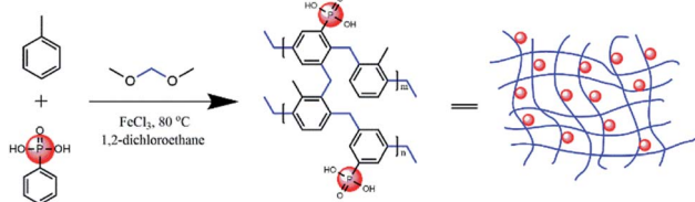
Fig. 1 Schematic of the preparation of PPOPs.
