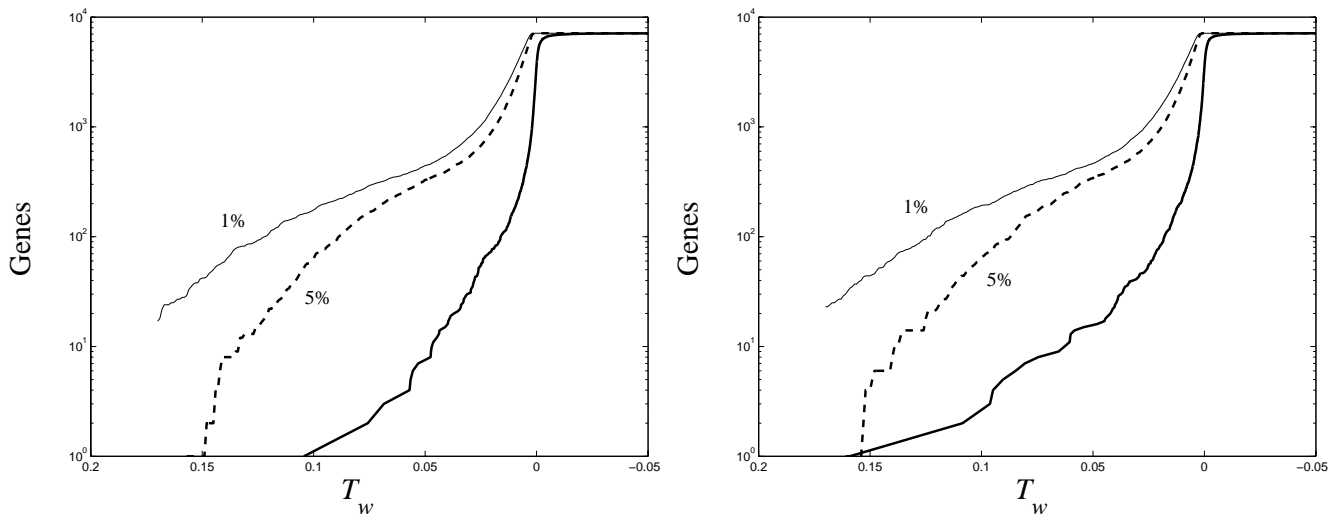
Figure 2 : Observed T_w(j) distribution computed on the Leukemia data set, compared to randomly per-mutated class distinctions. The number of genes highly expressed in a) ALL and b) AML is shown on y-axis.
