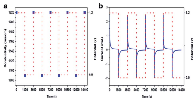
Fig. 5 (a) Salt water conductivity and (b) HCEDI current as function of time in response to cell charging at 1.2 V and discharging at 0 V in 30 mL of 10 mM NaCl electrolyte. Blue square represents measured conductivity; dotted line in red represents the charging–discharging procedure; blue line.
