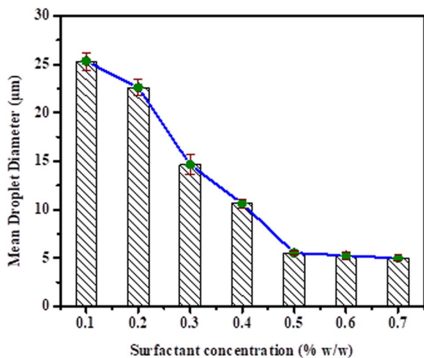
Fig. 2 Variation in droplet diameter of prepared emulsions with increasing concentration of saponin after 15 min of standing (calculated mean droplet diameter d_{32} 5.54 µm).
