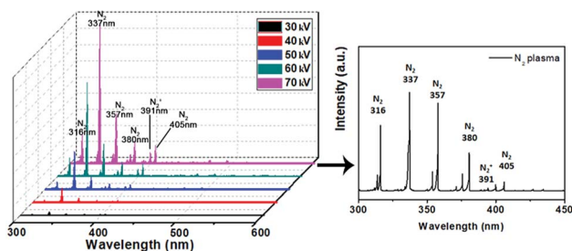
Fig. 2 OES of N_2 plasma in a DBD technique as a function of input voltage.
