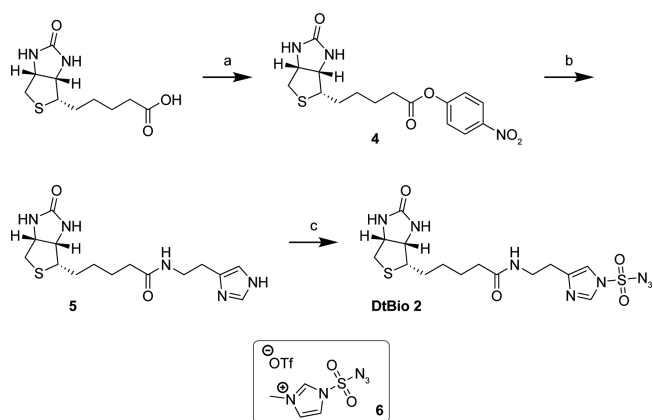
Figure 1. Top: structures of the nontargeted ( 1 ) and targeted ( 2 ) diazotransfer reagents and the boron–dipyrrromethene (BODIPY) fluorophore ( 3 ) used as reporter group in the evaluation of the diazotransfer reaction. Bottom: schematic representation of the targeted diazotransfer reaction concept. Ligands bearing the diazotransfer group direct the reagent to the protein of interest. Upon binding, an amino group of the protein is transformed into an azide in the presence of Cu(II). The modified protein can be further functionalized with bioorthogonal chemistry.
