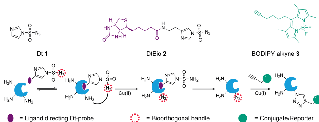
Figure 1. Top: structures of the nontargeted ( 1 ) and targeted ( 2 ) diazotransfer reagents and the boron–dipyrrromethene (BODIPY) fluorophore ( 3 ) used as reporter group in the evaluation of the diazotransfer reaction. Bottom: schematic representation of the targeted diazotransfer reaction concept. Ligands bearing the diazotransfer group direct the reagent to the protein of interest. Upon binding, an amino group of the protein is transformed into an azide in the presence of Cu(II). The modified protein can be further functionalized with bioorthogonal chemistry.
