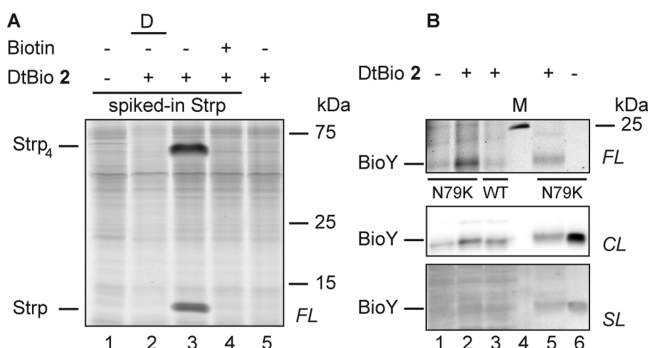
Figure 3. Labeling of streptavidin in E. coli lysates (A). A mixture of Strp (0.5 μg) and E. coli lysate (2.0 mg/mL) was incubated with DtBio 2 (10 μM). The modified proteins are visualized by clicking them to BODIPY-alkyne 3 subsequent to diazotransfer and resolving them on a 15% SDS-PAGE gel. (B) Cell surface labeling of N79K-BioY and wt-BioY. Cells expressing either form of BioY were treated with DtBio 2 (250 μM) in the presence of 1 mM CuSO 4 for 1 h, after which the modified proteins were clicked to 3. Labeling of BioY was visualized with fluorescence scanning (FL) of the lysate subsequent to cell disruption (top panel), detection of BioY subsequent to Western blotting of the same gel using HisProbe-HRP and chemiluminescence (CL) as a read-out (middle), and silver staining of the same gel post-transfer (lower panel) (lanes 1–3). To further confirm the labeling signal from N79K-BioY, the same sample as in lane 2 (B) was used for Ni-NTA bead purification of N79K-BioY, and the eluate is compared to untreated purified N79K-BioY (lanes 5 and 6).
