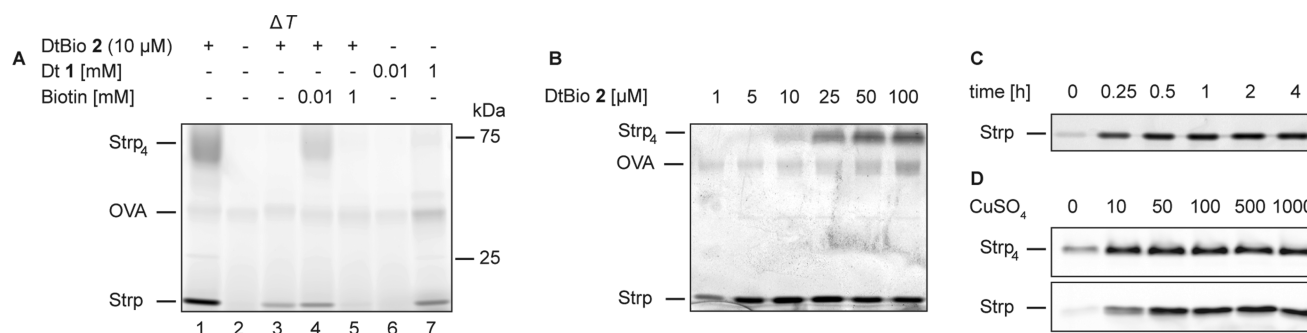
Figure 2. Biochemical evaluation of diazotransfer probe DtBio 2 with streptavidin (Strp) as target protein. (A) A mixture of Strp and OVA labeled with indicated amount DtBio 2 (lane 1) or Dt 1 (lanes 6 and 7) and clicked to BODIPY-alkyne 3 subsequent to diazotransfer is resolved on a bis-tris 4–12% gradient gel and visualized by fluorescence scanning. Heat-inactivation with 1% SDS prior to incubation (lane 3) and competition with D-biotin (lanes 4 and 5) were used as controls. Note: biotin and derivatives thereof (such as DtBio 2) stabilize tetrameric Strp. (B) A mixture of streptavidin and OVA was incubated with indicated amount of DtBio 2, after which the modified proteins were visualized as described above (resolved on a 15% Laemmli type SDS-PAGE gel). (C) Crop showing the labeling intensity of monomeric streptavidin incubated with DtBio 2 (10 \mu M) for the indicated time, after which the modified proteins were visualized as described above. (D) Crops showing the labeling intensity of tetrameric and monomeric streptavidin incubated with DtBio 2 (10 \mu M) in the presence of the indicated amount ( \mu M) of CuSO 4 , after which the modified proteins were visualized with dibenzylcyclooctyne–tetramethylrhodamine 7. For uncropped images and coomassie brilliant blue (CM) staining of the gels, see Figures S1–4.
