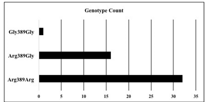
Fig. 1. Prevalence of genotype in patients with evidence of dual atrioventricular nodal pathways.
