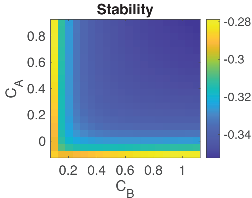
Appendix 1—figure 2. Stability analysis of the system. Plot shows for a range of values for C_A and C_B the negative of the maximum real part of all the eigenvalues of \mathbf{A}(-\text{Re}(\lambda)) , see details above). Negative values indicate that the system's state is stable. We choose values for k and l_T to be as given in Table 1 .
