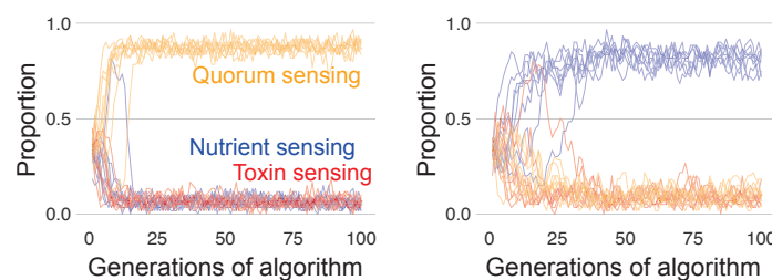
Appendix 1—figure 10. The benefit of toxin sensing over other sensing strategies is lost when competition time is short. As in Figure 4c , we pit all three sensory strategies against each other in a Appendix 1—figure 10 continued on next page
