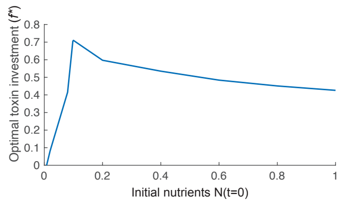
Appendix 1—figure 3. The effect of nutrient availability on optimal toxin investment. We plot the evolutionary stable investment into toxin over a range of different initial levels of nutrient ( N(t=0) ). The optimal investment is highest for an intermediate amount of nutrients. Other parameters of the model take the standard values given in Table 1 .
