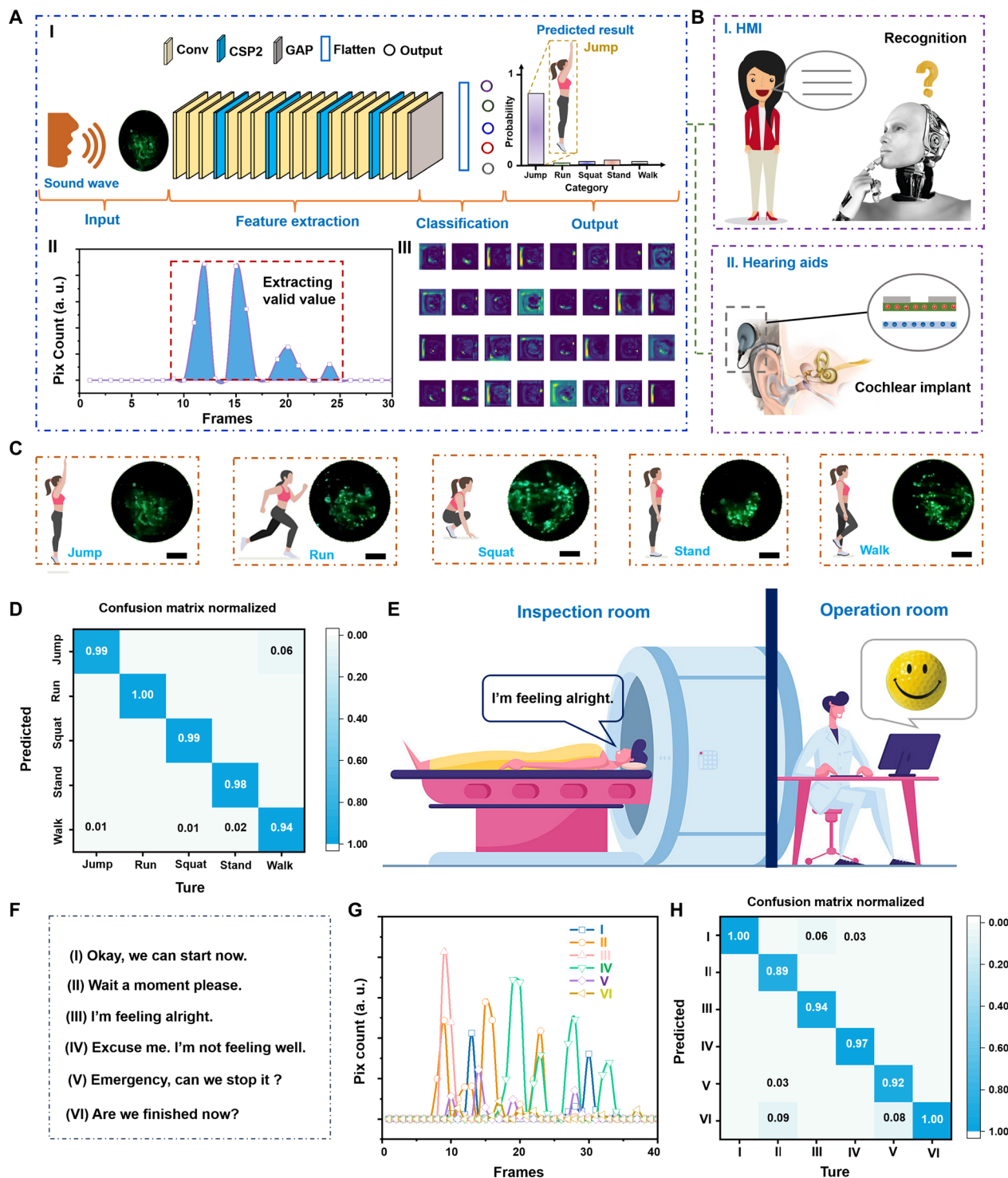
Fig. 5. The speech recognition application of SVTAS. (A) Illustration of CNN for speech recognition. (I) Structure of CNN, (II) luminescent pix count from SVTAS in typical image sequence, and (III) visualization of luminescence features extracted by CNN. (B) Proposed application of SVTAS in (I) HMI and (II) hearing aids. (C) A typical exemplary set of the actual luminescent images of SVTAS corresponding to the five command words. Scale bars, 1 cm. (D) Classification test normalized confusion matrix for recognizing the five words in (C). (E) Proposed application of SVTAS in nuclear magnetic resonance scan. (F) Six sentences of patient demand and (G) luminescent pix count from SVTAS corresponding to six sentences. (H) Classification test normalized confusion matrix for recognizing the six sentences in (F).
