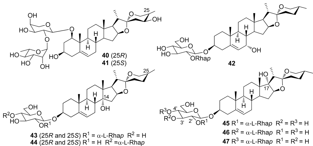
Figure 3. Chemical structures of spirostanol diglycosides isolated from Dracaena and Sansevieria species.
