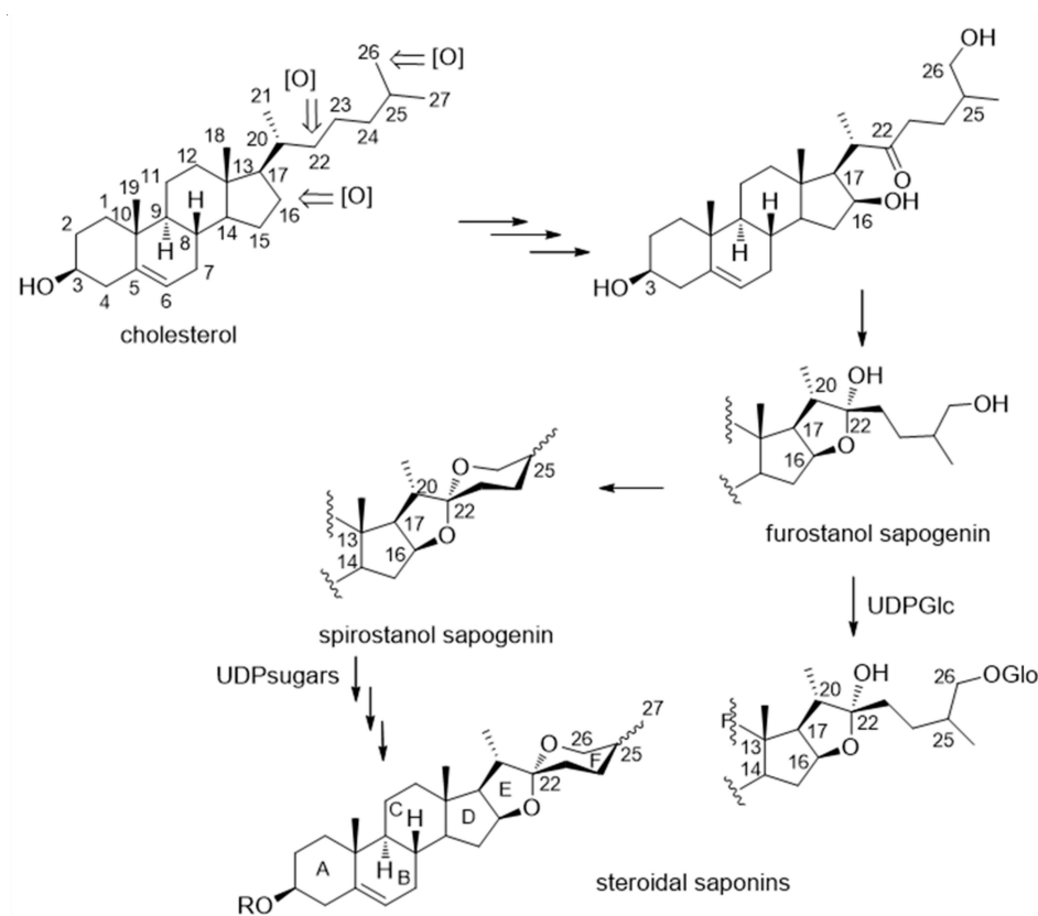
Figure 1. Main steps in the biosynthetic transformation of cholesterol to steroidal saponins.
