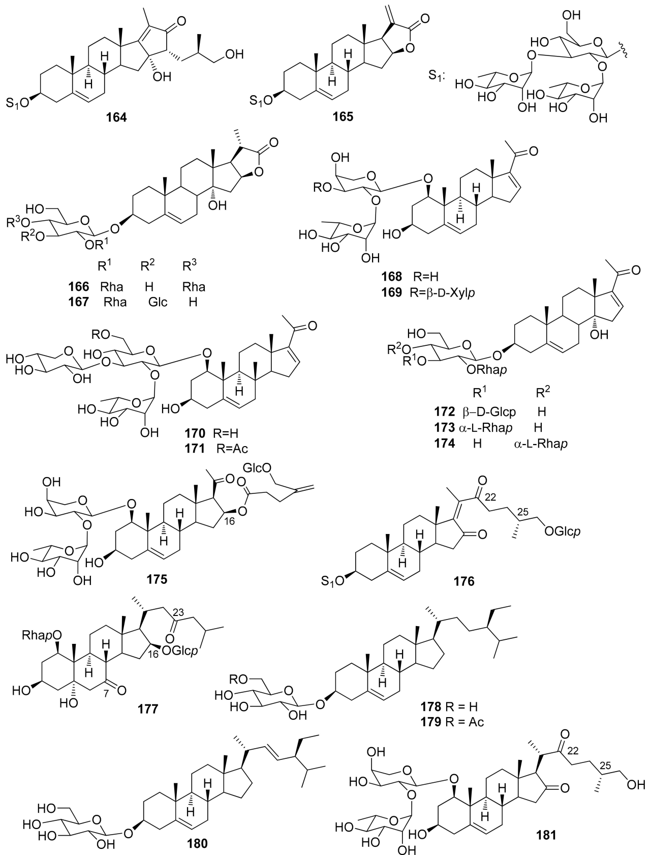
Figure 9. Chemical structures of miscellaneous steroidal saponins isolated from Dracaena and Sansevieria species.
