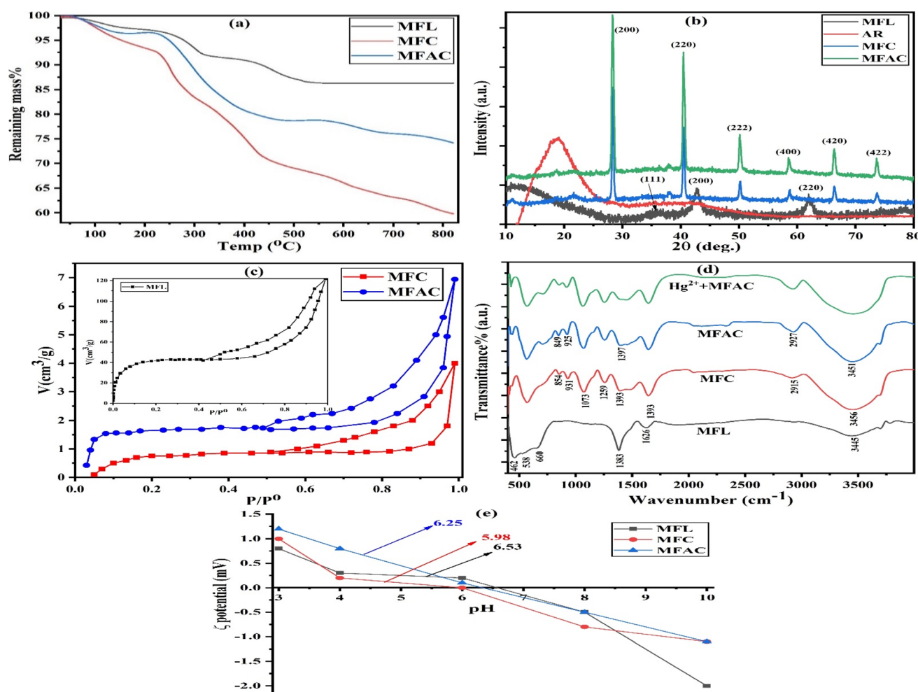
Fig. 1 TGA (a), XRD (b), \text{N}_2 adsorption (c), ATR-FTIR (d), zeta potential (e) curves for MFL, MFC, and MFAC, additionally, XRD for AR gum and ATR-FTIR curve of MFAC after \text{Hg}^{2+} adsorption.
