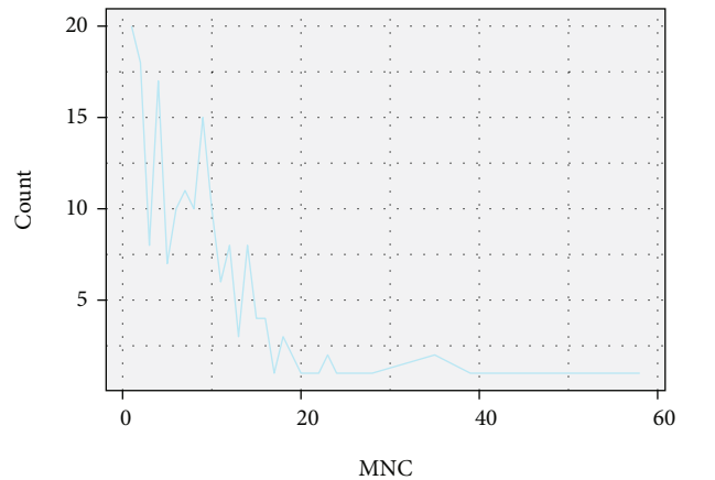
FIGURE 4: PPI network analysis and key genes' recognition. (a) PPI network for DEGs. Red rectangle node: upregulated genes; green rectangle node: downregulated genes. (b) Key genes were screened using Cytoscape cytoHubba plugin based on the four methods, Degree, Betweenness, Closeness, and MNC. PPI: protein-protein interaction.
