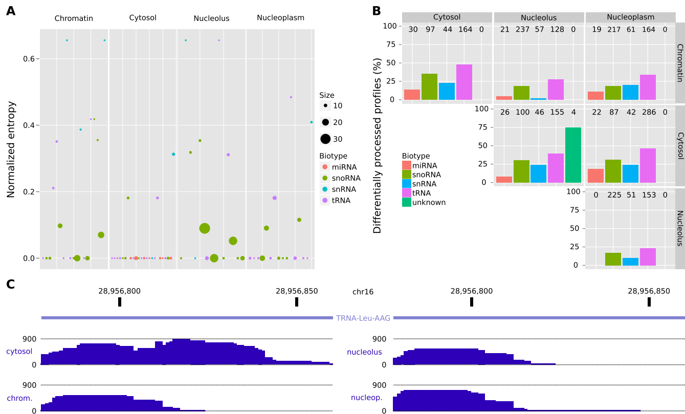
Figure 4. Differential processing across ENCODE cell compartments. (A) Representation of clusters containing five or more sncRNAs across all four ENCODE cell compartments. The size of the points represents the number of sncRNAs from the extended annotation contained in the cluster. The normalized entropy ( y -axis) represents the purity of a cluster (Supplementary Materials and Methods), the lower the entropy, the higher the purity of the cluster. (B) Proportion of profiles from the extended annotation that are differentially processed between cellular compartments separated by non-coding RNA family ( y -axis). Numbers at the top of the bars represent the total number of profiles detected in both compartments. (C) Representation of the read profiles for the tRNA-Leu-AAG transfer RNA showing abundant processing of the 3'-half in the cytosol compared to the chromatin compartment. The plot represents the number of reads per nucleotide in the same scale for each compartment.
