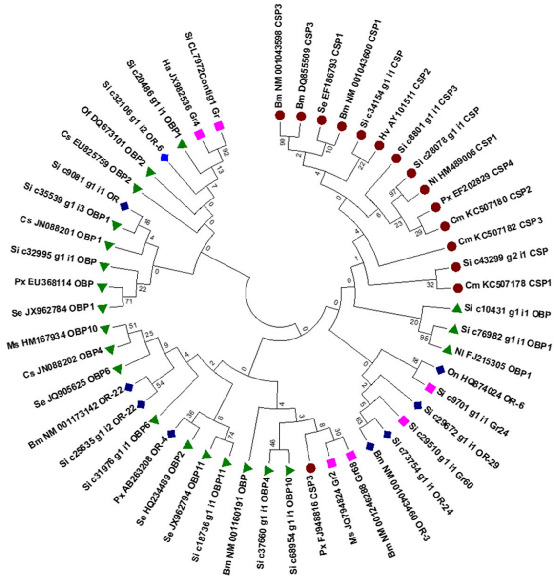
Figure 6 Phylogenetic tree for annotated sequences of chemoreception mechanism among S. incertulas (Si), lepidopteran, and hemipteran insects. Bm, B. mori ; Cm, Cn. medinalis ; Cs, C. suppressalis ; Ha, H. armigera ; Hv, He. virescens ; Ms, M. sexta ; Ni, N. lugens ; On, O. nubilalis ; Of, O. furnacalis ; Px, P. xylostella ; Se, S. exigua .
