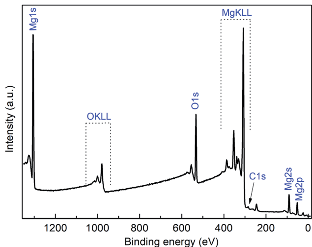
Fig. 10 XPS spectra of the MgO film obtained from 3a at 450 °C ( N_2 , 50 mL \text{min}^{-1} ; after 2 min sputtering, Ar^+ , 4.0 keV).
