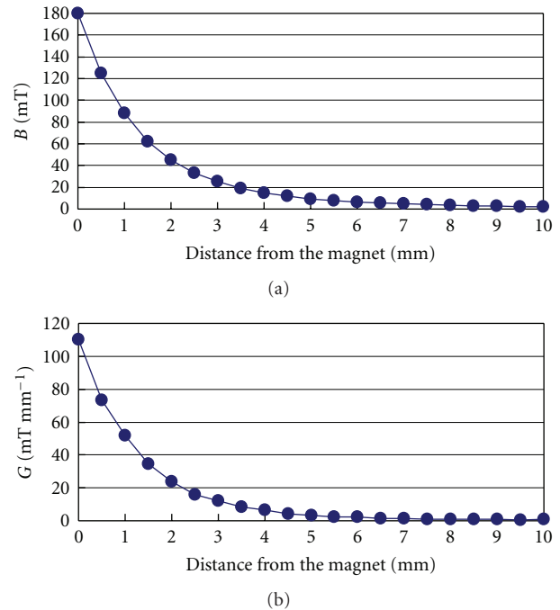
FIGURE 1: (a) Spatial distribution of the magnetic flux density values. (b) Spatial distribution of the magnetic gradient values.
