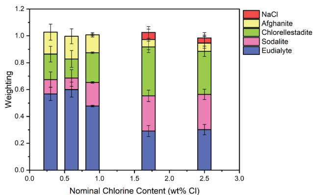
Fig. 8 The mean weighted contributions of XANES data from reference compounds NaCl, afghanite, chlorellestadite, sodalite and eudialyte, required to fit the data of glass-ceramic sample compositions A–E; see text for discussion.
