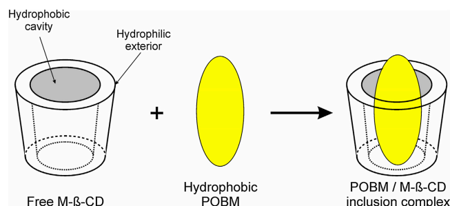
Figure 15. Schematic illustration of the association of free methyl- \beta -cyclodextrin and POBM to form a 1:1 inclusion complex. Reprinted from [32]. Copyright (2018), with permission from Elsevier.
