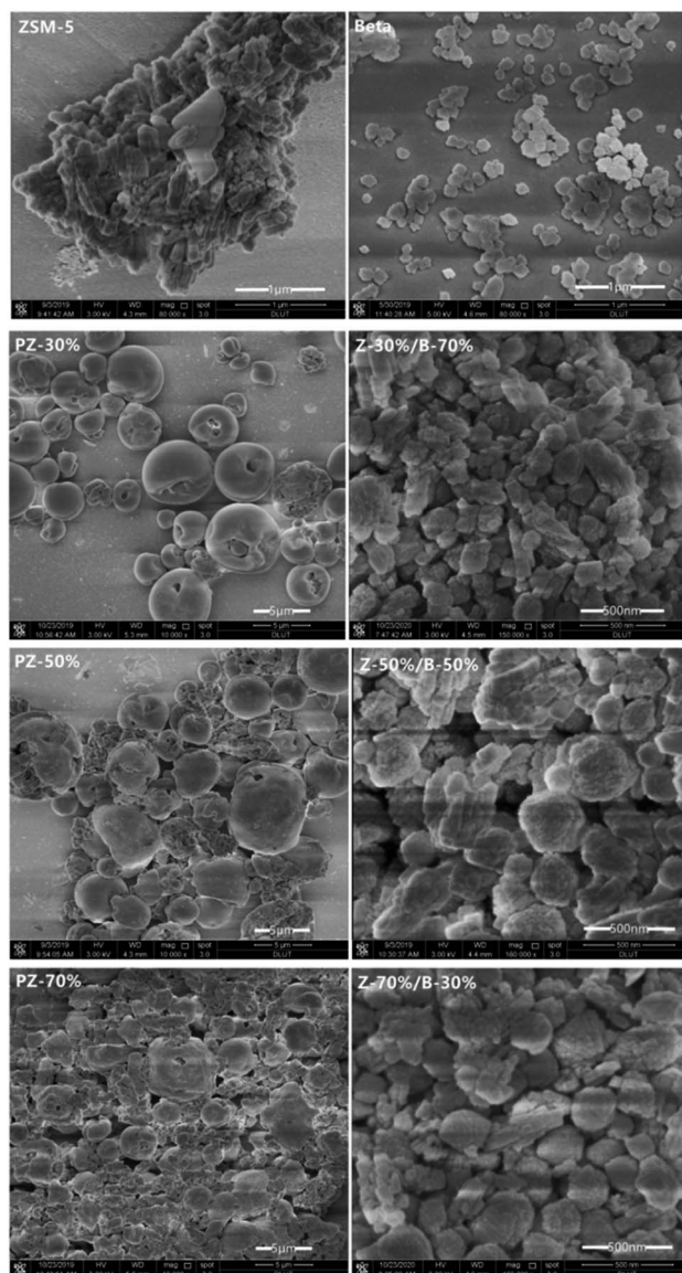
Fig. 13 SEM images of: pure ZSM-5 and beta zeolite; the PZ- x samples; the Z- x /B- y samples with different mass ratios.
