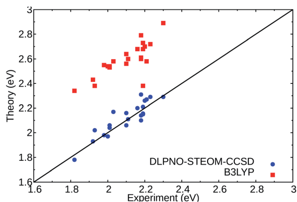
Fig. 2 Comparison of the experimental absorption band maxima and the computed vertical excitations for the lowest 1A → 2A states of the selected DASAs 21,22 (Fig. S1 and Table S1†) for DLPNO-STEOM-CCSD (blue circles) and TDDFT (B3LYP) (red squares) in gas phase. The black line signifies a perfect agreement between theory and experiment.
