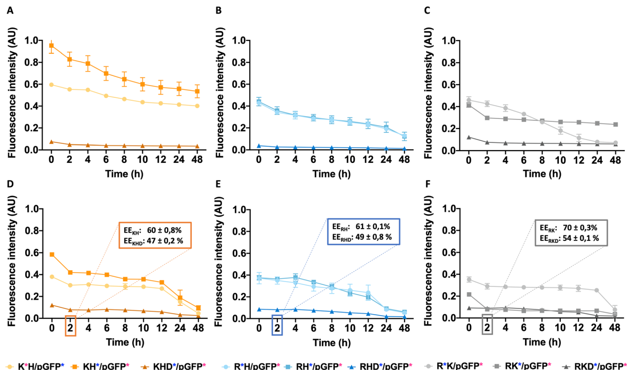
Fig. 7 Nanoparticles demonstrate stability at different temperatures. Cationic and anionic coated nanoparticle FRET values, incubated with FBS: From A to C at 25 °C and from (D)–(F) at 37 °C. In (A) and (D) KH and KHD constructs, in (B) and (E) RH and RHD constructs and in (C)–(F) RK and RKD constructs are represented. In figures (D)–(F) there are amplifications indicating the EE% of the nanoparticles after 2 h of incubation at 37 °C.
