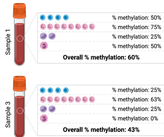
Fig. 2. Sources of variation in DNA methylation in heterogeneous tissues. A) Samples 1 and 2 differ in overall DNA methylation because of changes in proportions of cell types. Individual cell types do not differ in DNA methylation levels among the two samples. B) Samples 1 and 3 differ in overall DNA methylation because of changes in DNA methylation levels of individual cell types. The proportion of each cell type are not different in the two samples. Image created with BioRender ( biorender.com ).
