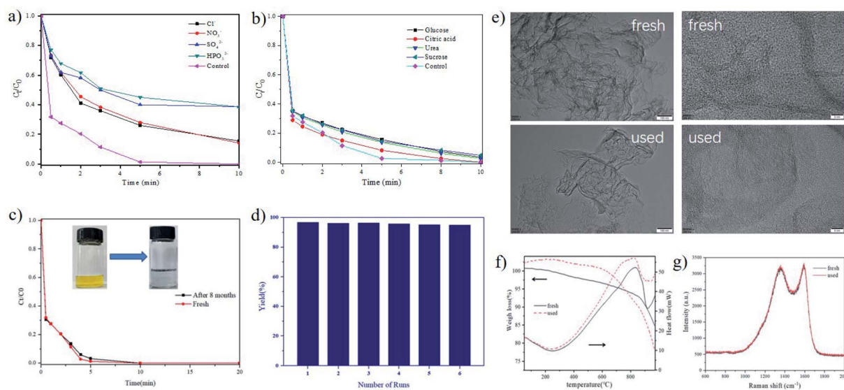
Fig. 7 Interferences, stability, and renewability of N@C-g-C 3 N 4 -950. (a) Effects of ions; (b) effects of organic compounds; (c) store stability after 8 months; (d) operational stability after 6 cycles; (e) TEM images of fresh and used catalyst; (f) TGA curves of fresh and used catalyst; (g) Raman curves of fresh and used catalyst. Reaction conditions: 25 mL K 2 Cr 2 O 7 (0.68 mM), 1 mL HCOOH (98%), 25 mg catalyst, room temperature, and stirring rate 500 rpm.
