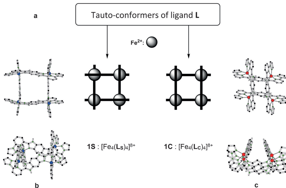
Figure 2. The coordination of L to Fe II metal ions leads to the tautomerism-driven emergence of complexity. a) Schematic representation of the cationic moieties of the isolated isomers of the [2 × 2] Fe II 4 grid complexes, consisting of L (black bars) and Fe II ions (gray spheres). The molecular structures of the two [Fe 4 L 4 ] 8+ tauto-conformers were determined by single-crystal X-ray diffraction. b) Top and side view of 1S , c) top and side view of 1C (C black, Fe HS red, Fe LS blue, N green).
