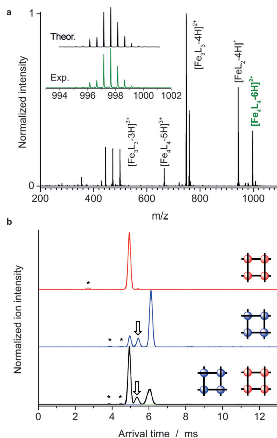
Figure 3. IM-MS analysis to distinguish the isomeric complexes (with identical m/z ratios). a) Mass spectrum (reaction solution) of 1 ; peaks that are due to [\text{Fe}_4\text{L}_4-6\text{H}]^{2+} are shown in green. b) Arrival time distributions (ATDs) for [\text{Fe}_4\text{L}_4-6\text{H}]^{2+} : 1C (top, in red), 1S (middle, in blue), and the as-synthesized mixture (bottom, in black); the arrows indicate an intermediate species ( IS , for details see SI7).
