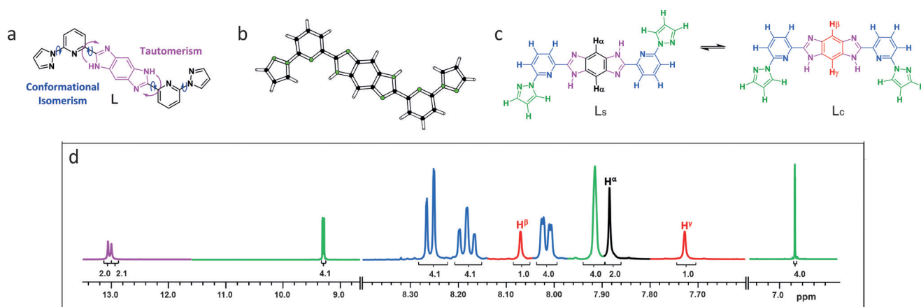
Figure 1. a) The conformational isomerism and tautomerism of L . b) Molecular structure of L S as determined by single-crystal X-ray diffraction (C black, H white, N green). c) The resulting L S and L C conformers of L as found in solution. d) 1 H NMR spectrum (in [D 6 ]-DMSO) showing the presence of L S and L C in a 1:1 ratio. The protons were assigned using the color codes shown in (c) and (d).
