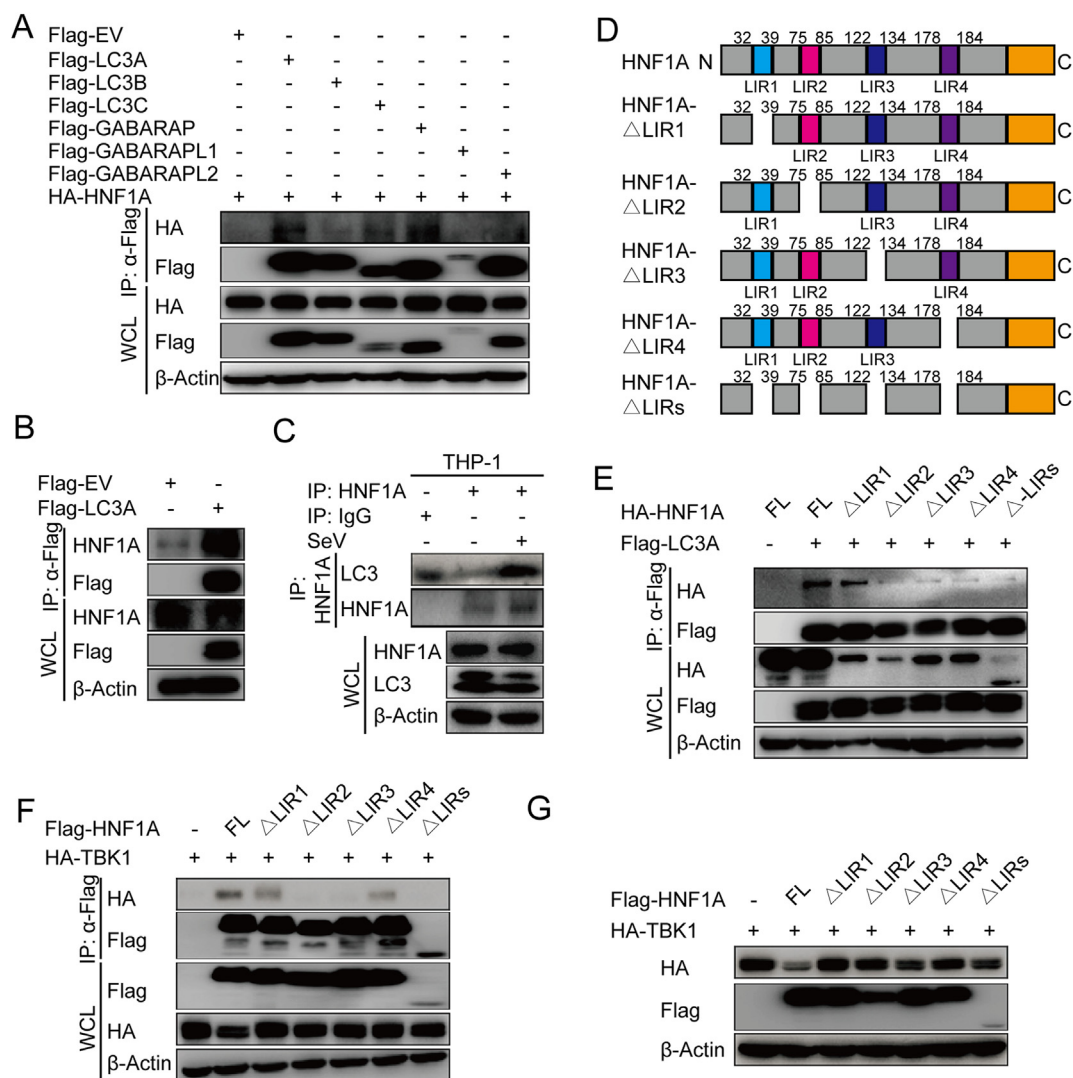
Figure 6 HNF1A can bind to LC3 through its LIR docking sites. (A) 293T cells transfected with HA-HNF1A together with Flag-EV, Flag-LC3A, Flag-LC3B, Flag-LC3C, Flag-GABARAP, Flag-GABARAPL1 or Flag-GABARAPL2. After immunoprecipitation with anti-Flag beads and immunoblot analysis. (B) 293T cells transfected with Flag-EV or Flag-LC3A, followed by immunoprecipitation (IP) with anti-Flag beads and immunoblot analysis. (C) THP-1 cells infected with SeV for 24 h, followed by immunoprecipitation (IP) with anti-HNF1A and immunoblot analysis. (D) Schematic diagrams of HNF1A, HNF1A-ΔLIR1, HNF1A-ΔLIR2, HNF1A-ΔLIR3, HNF1A-ΔLIR4, HNF1A-ΔLIRs. (E) Immunoprecipitation analysis of the interaction between HNF1A and LC3A or its mutants in 293T cells. (F) Immunoprecipitation analysis of the interaction between HNF1A and TBK1 or its mutants in 293T cells. (G) Immunoblot analysis of 293T cells transfected with deletion mutants of HNF1A together with HA-TBK1.
