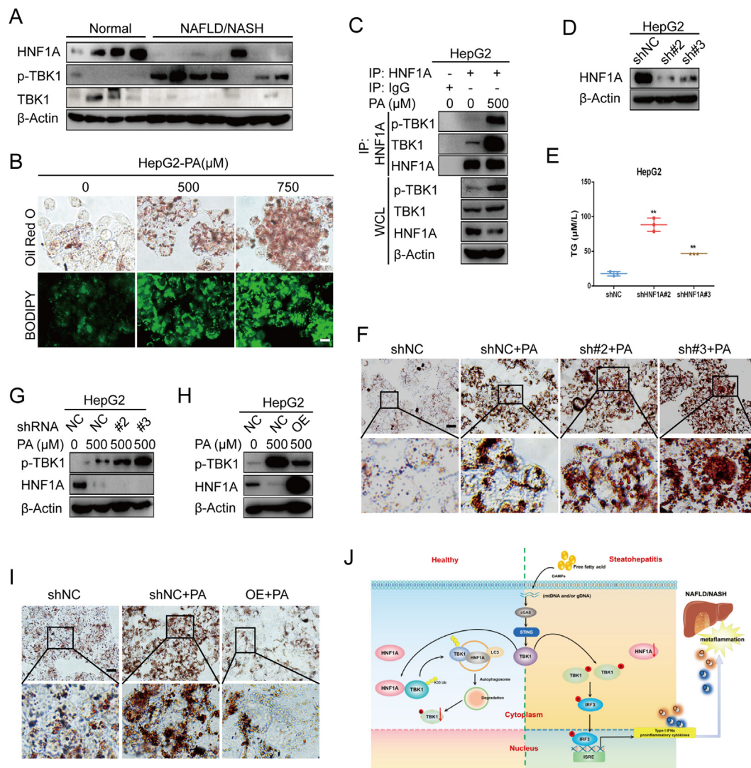
Figure 8 HNF1A ameliorates NAFLD/NASH via targeting active TBK1. (A) Immunoblot analysis of phosphorylated TBK1 (p-TBK1) and HNF1A in NAFLD/NASH and normal clinical specimens. (B) Representative Oil Red O or BODIPY staining in HepG2 cells challenged with palmitate for 24 h. Original magnification, 20 \times . (C) HepG2 cells treated with BSA or BAS-palmitate for 24 h, followed by immunoprecipitation with anti-HNF1A and immunoblot analysis with p-TBK1 and TBK1. (D) HNF1A knockdown (KD) in HepG2 cells at protein levels. (E) Triglyceride content quantification in shNC or HNF1A KD HepG2 cell lysates. (F) Representative Oil Red O staining in shNC or HNF1A KD HepG2 cells treated with BSA or BSA-palmitate for 24 h. Original magnification, 20 \times . (G) Immunoblot analysis of phosphorylated TBK1 (p-TBK1) and HNF1A in shNC or HNF1A KD HepG2 cells treated with BSA or palmitate for 24 h. (H) Immunoblot analysis of phosphorylated TBK1 (p-TBK1) and HNF1A in shNC or HNF1A overexpression (OE) HepG2 cells treated with BSA or BSA-palmitate for 24 h. (I) Representative Oil Red O staining in shNC or HNF1A overexpression (OE) HepG2 cells treated with BSA or BSA-palmitate for 24 h. Original magnification, 20 \times . (J) Schematic representation of HNF1A-mediated innate immune responses in the pathogenesis of NAFLD/NASH.
